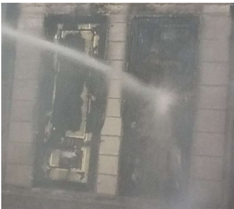
Fig. 6 Exposed Side during Hose Stream Test
