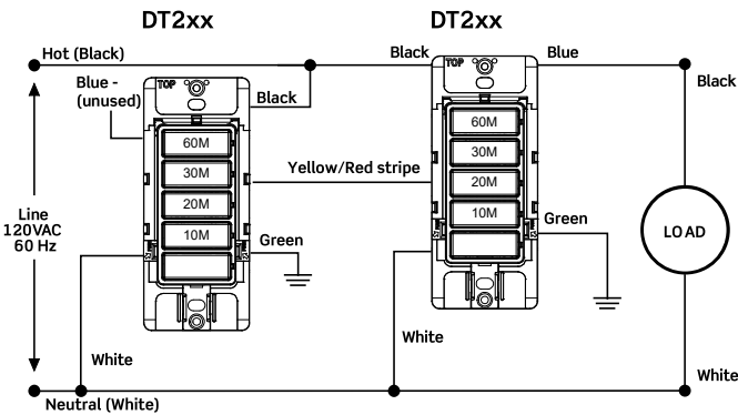
3-Way with Two DT2xx Timers
